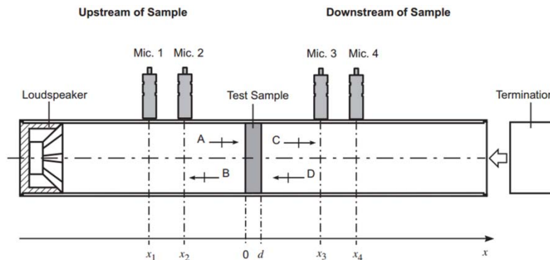
Source: Product data sheet: Transmission Loss Tube Kit (50 Hz – 6.4 kHz) Type 4206-T, Brüel & Kjær, 2012-09
