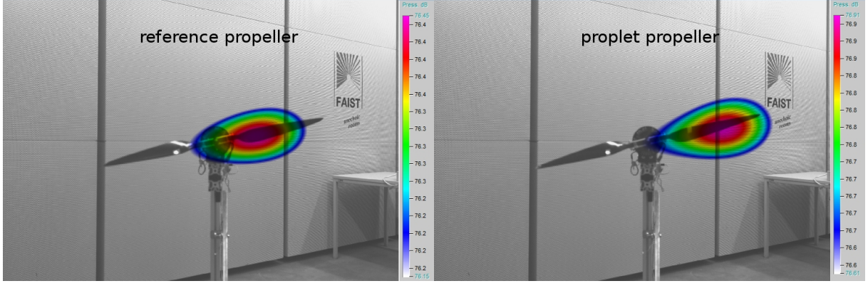
Figure 4: Acoustic images of both propellers at 800 Hz third octave band
