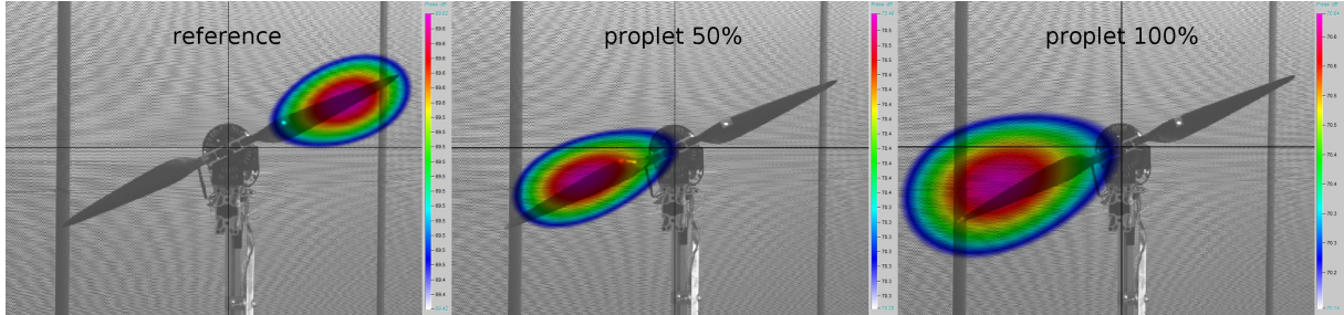
Figure 8: Acoustic images of the propellers at 800 Hz third octave band
