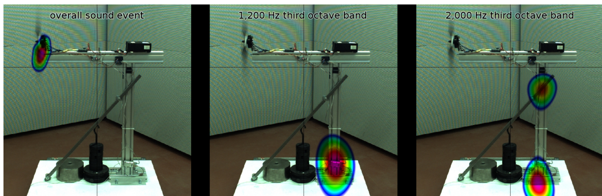
Figure 12: Acoustic images of the test bench - overall sound event; 1,200 Hz & 2,000 Hz third octave bands
