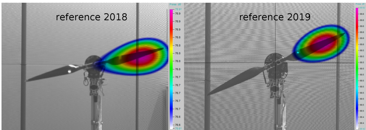
Figure 7: Acoustic images of reference propeller at 800 Hz third octave band - 2018 vs. 2019
