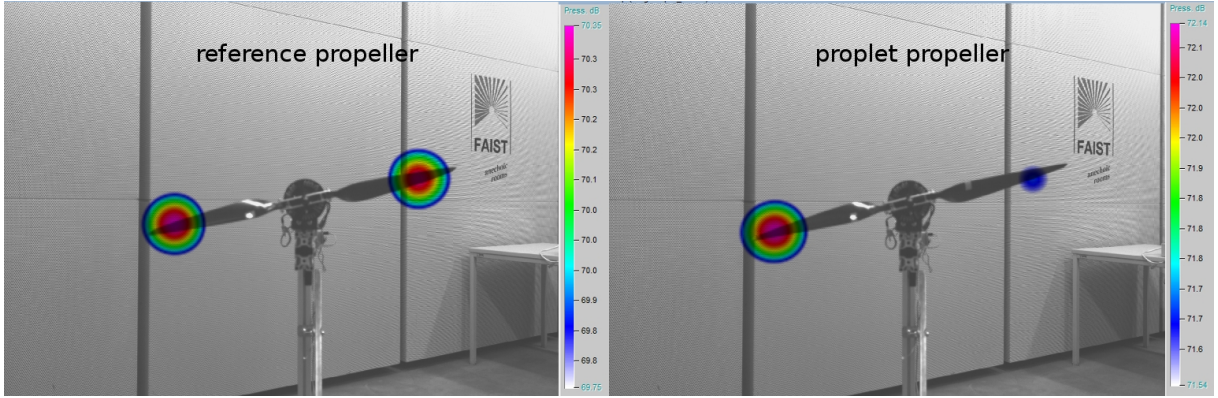
Figure 5: Acoustic images of both propellers at 1,600 Hz third octave band
