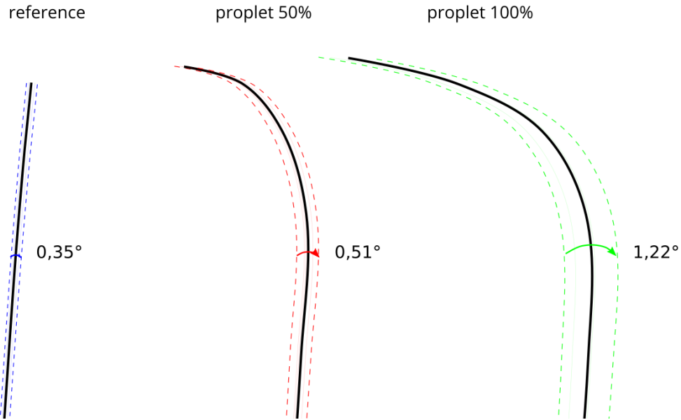
Figure 11: Comparison of the propeller's angles of deflection
