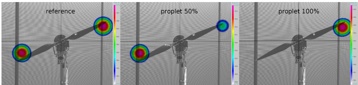
Figure 9: Acoustic images of the propellers at 1,600 Hz third octave band
