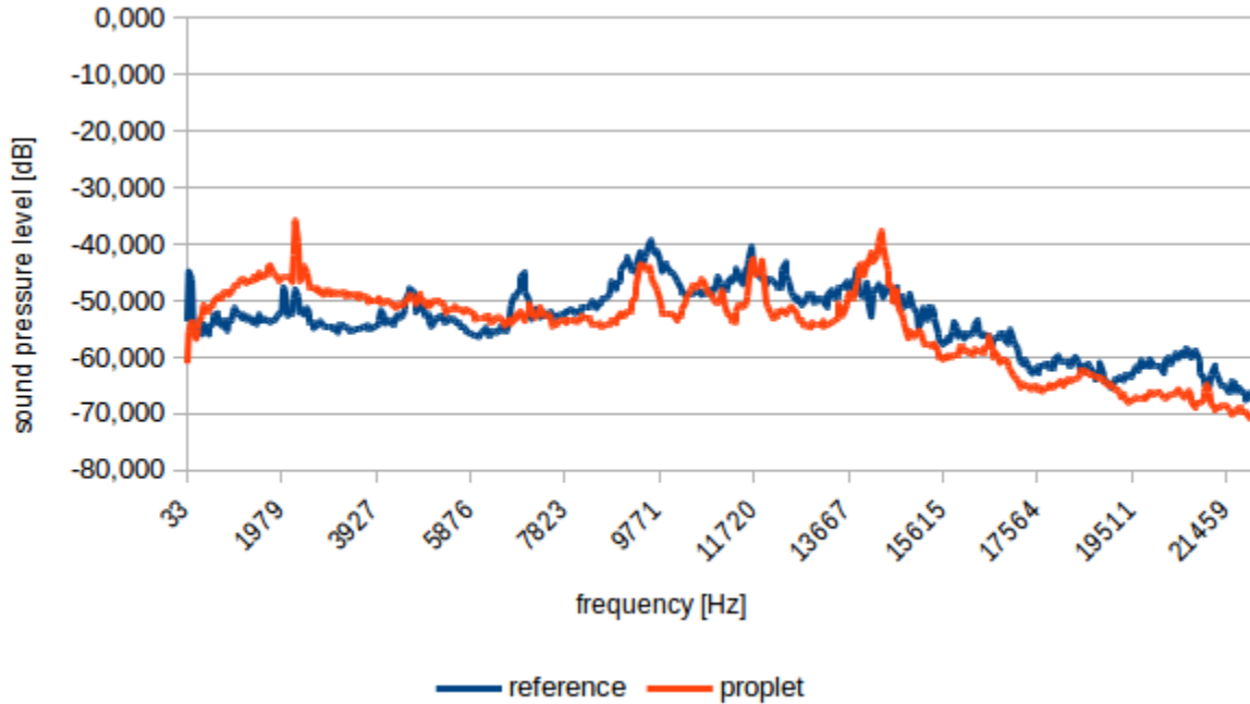
Figure 3: Frequency response analysis (linear depiction)
