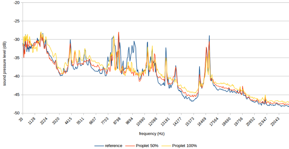
Figure 6: Frequency response analysis (linear depiction)
